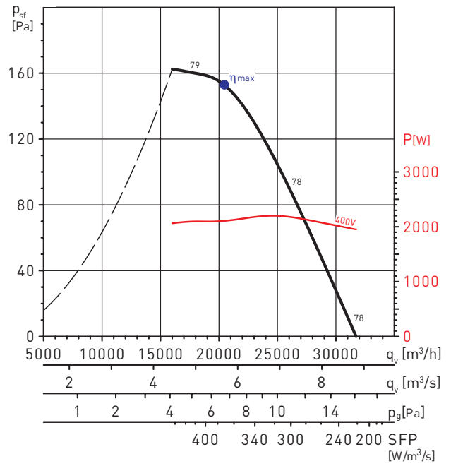
HCFT/6-900/H
