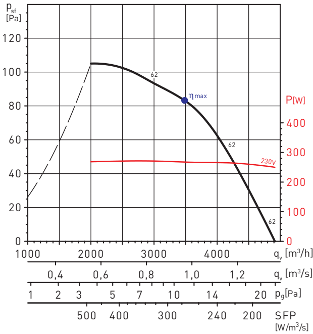
HCFB/4-400/H
