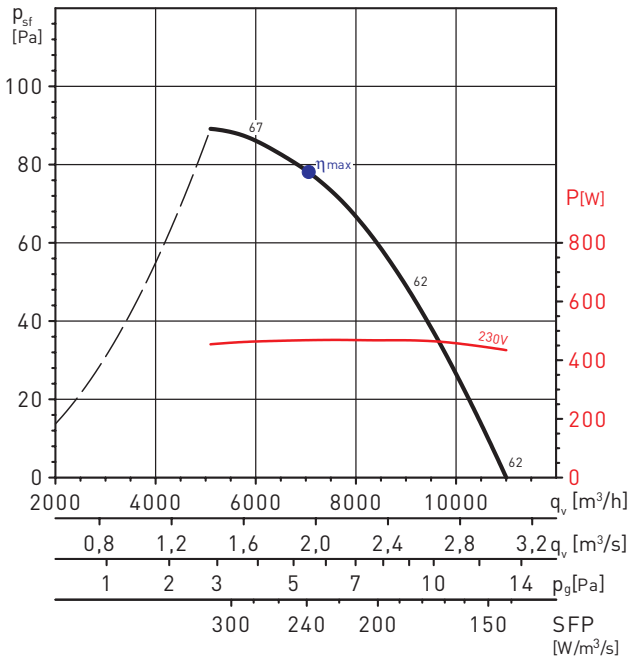
HCFB/6-630/H
