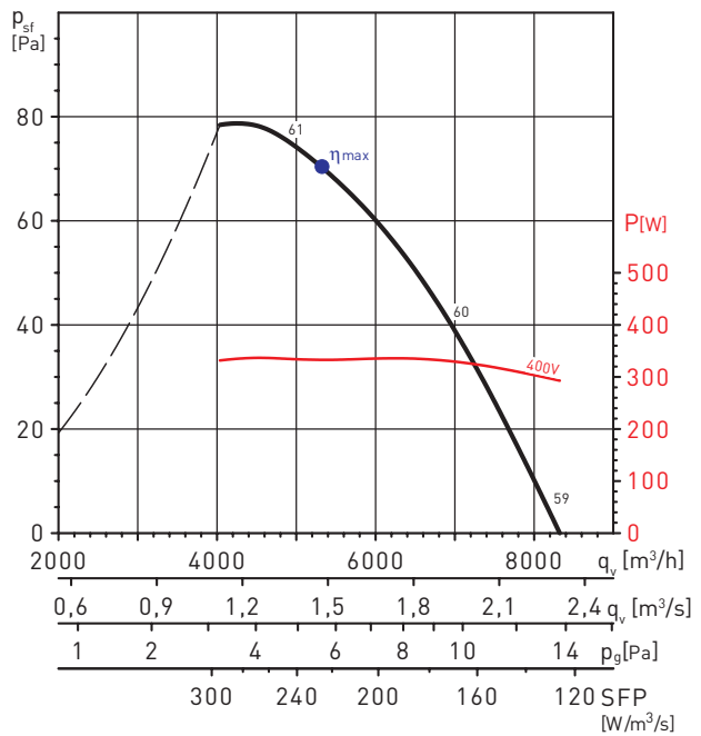
HCFT/6-560/H
