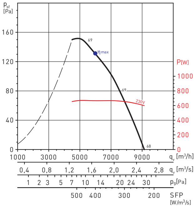
HCFB/4-500/H
