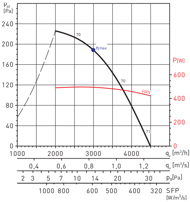
HCGT/2-355/I
