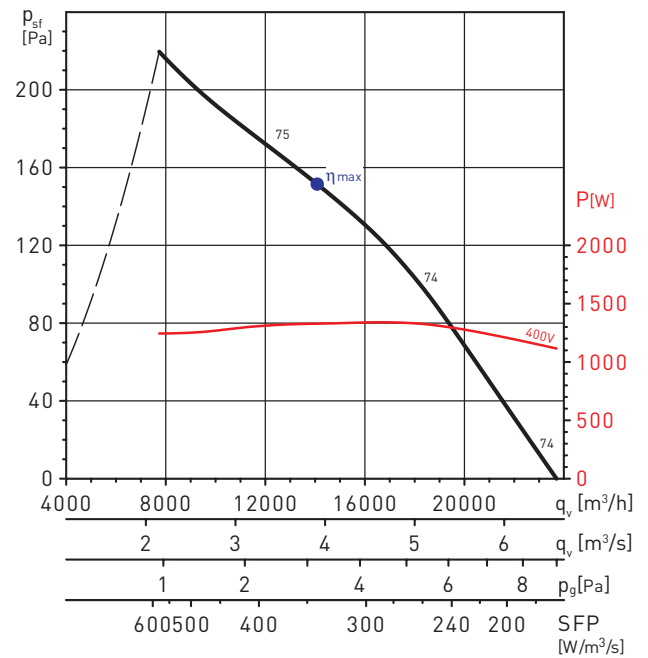
HCBT/6-900/L
